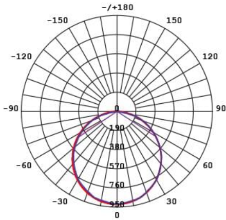
S9784U312TC at 4000K
