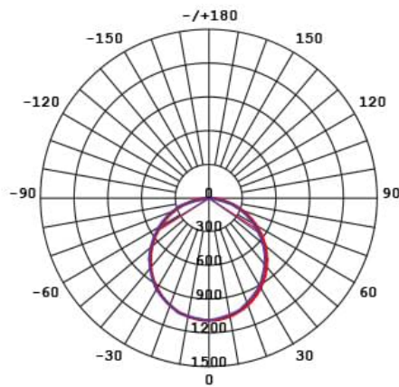
S9784U606TC at 5000K
